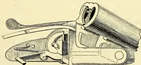
Combined Lever and Barrel-cocking Hammerless Mechanism.
